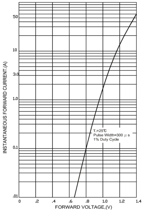
FIG.3-TYPICAL FORWARD CHARACTERISTICS
